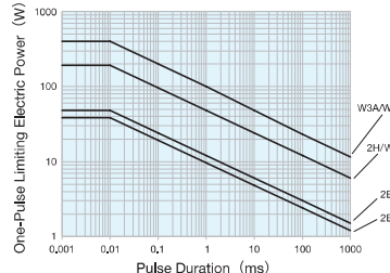
RK73B 2B-W3A2
